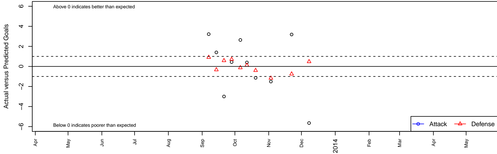
Evergreen United Earthquakes Blue B02 Dots are actual minus expected GF (blue circles) and GA (red triangles). Blue line is smoothed change in attack strength. Red is smoothed change in defense strength.
